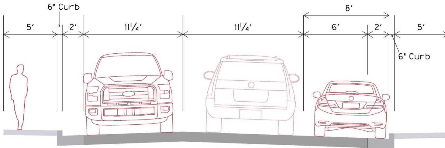
WALKERTOWN TYPICAL SECTION WITH ON-STREET PARKING
