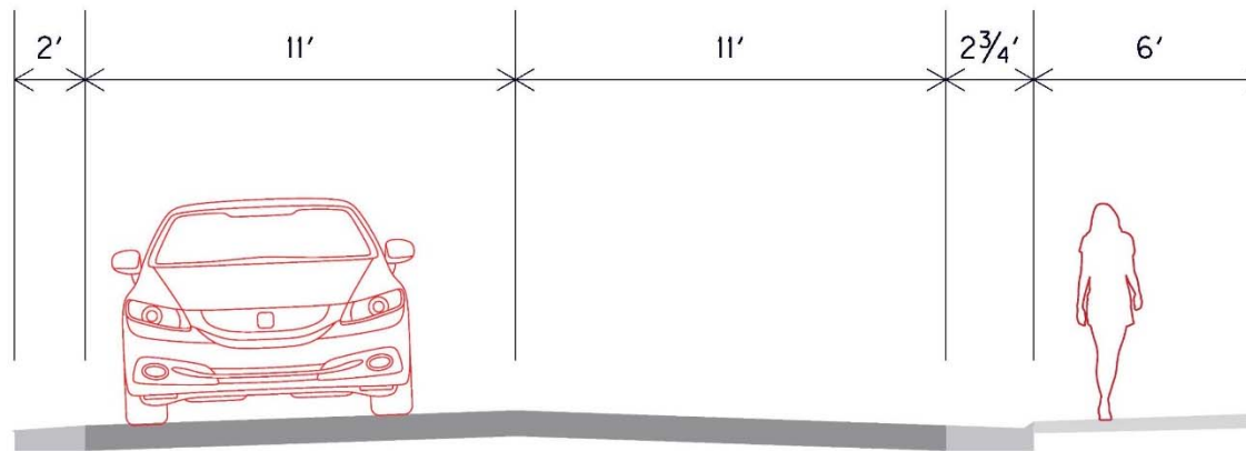
WABACO TYPICAL SECTION
